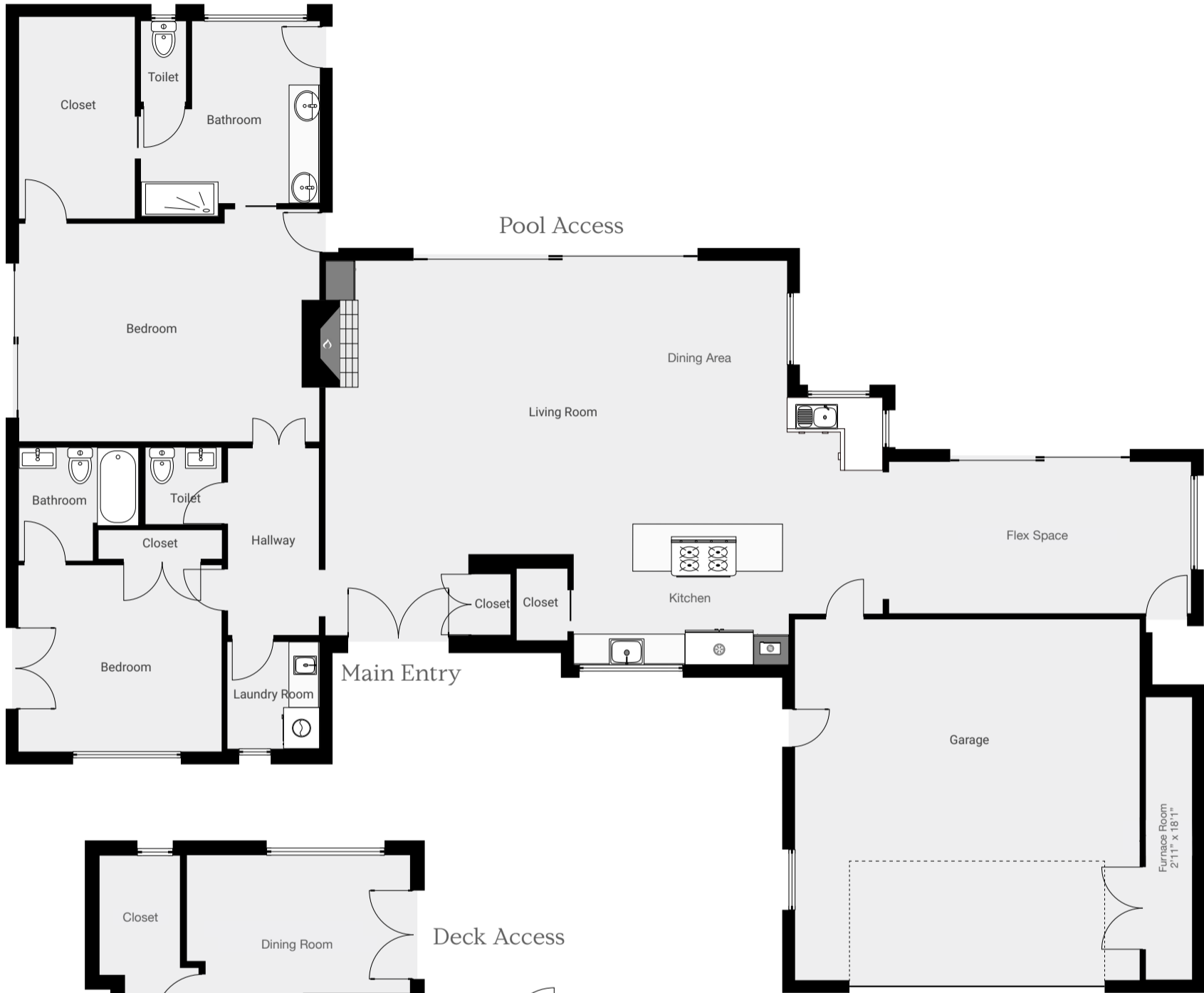
Main Floor
